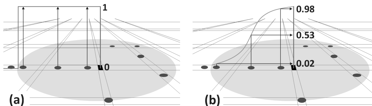
Figure 1 IVA Analysis Diagram
