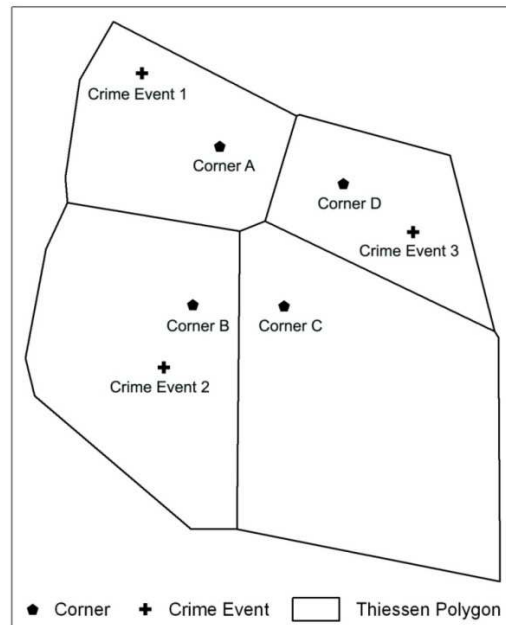
Figure 3 Example of Thiessen Polygon
